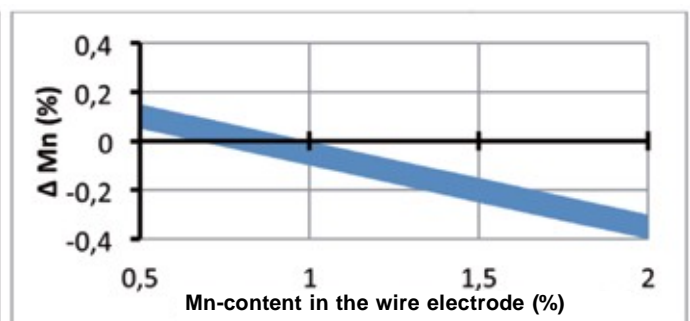
Pick-up/Burn-out Manganese
